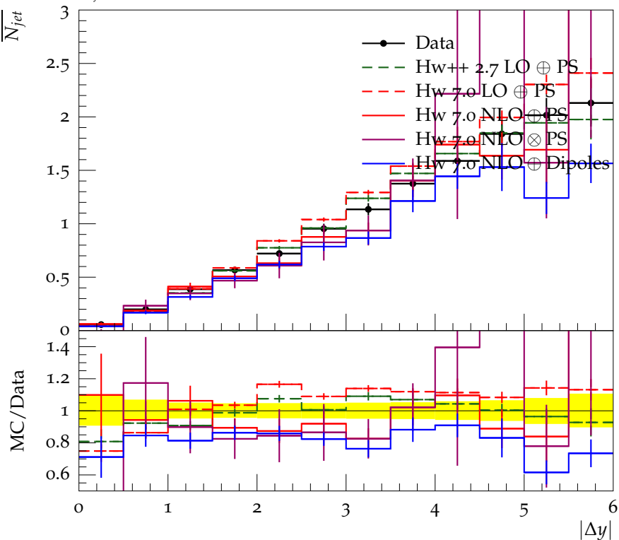
\overline{N}_{jet} vs |\Delta y| for 120 < \overline{P}_T < 150 , Fwd/Bwd
