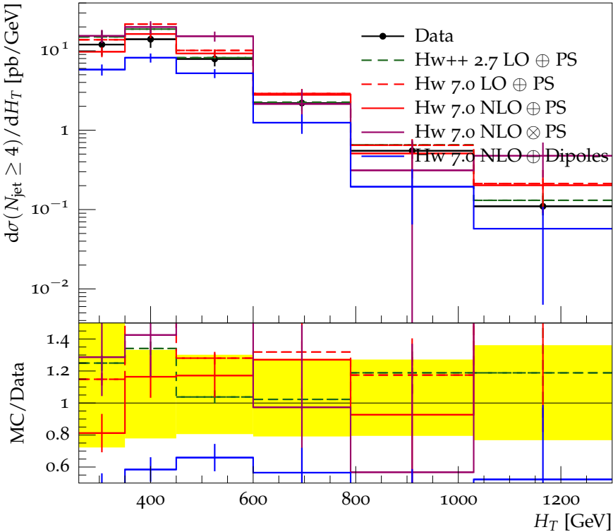
H_T for events with N_{\text{jet}} \geq 4 ( R = 0.4 )
