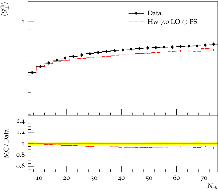
Average transverse sphericity vs. multiplicity
