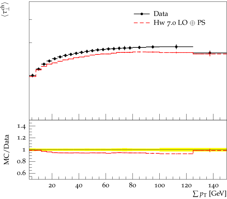
Average transverse thrust vs. transverse \sum p_T
