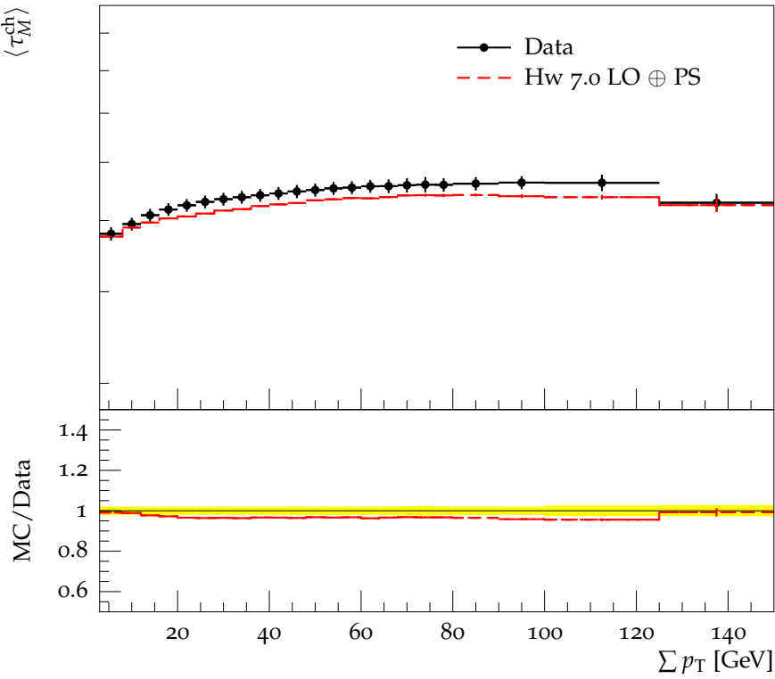
Average transverse thrust minor vs. transverse \sum p_T
