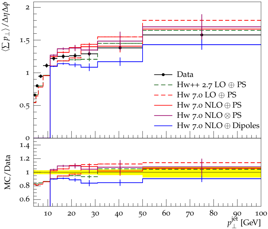
Mean \Sigma p_{\perp} vs. leading jet p_{\perp} , R = 0.6 , Transverse region
