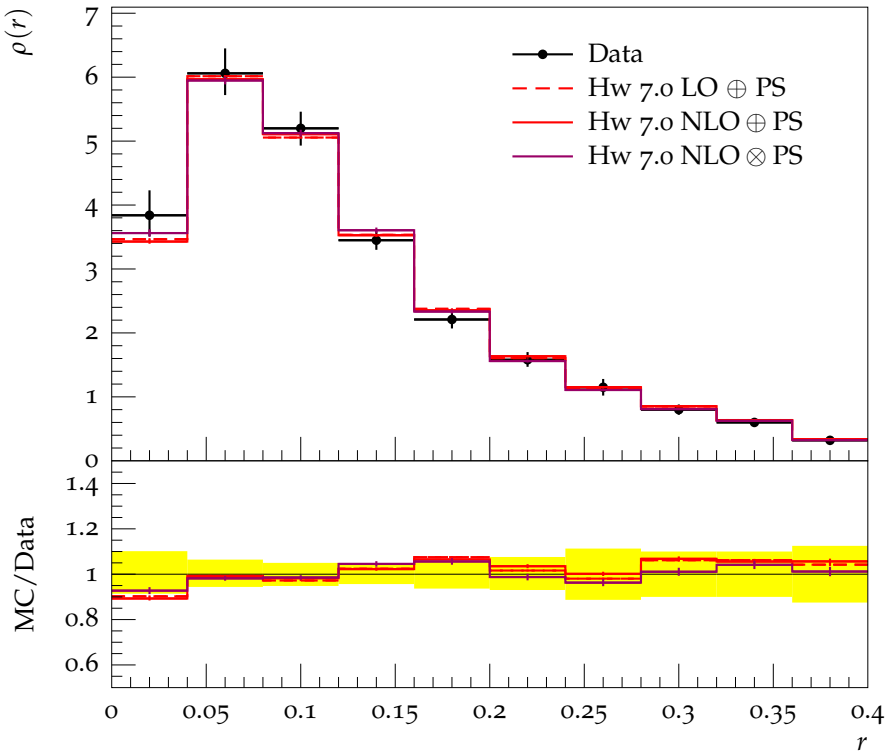
Differential jet shape for b -jets with 30 \text{ GeV} < p_T < 40 \text{ GeV}
