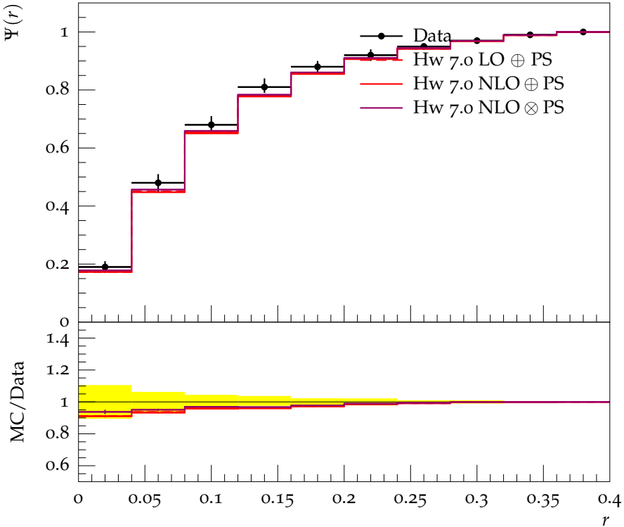
Integrated jet shape for b -jets with 40 \text{ GeV} < p_T < 50 \text{ GeV}
