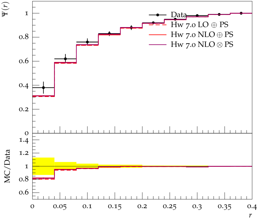
Integrated jet shape for light jets with 40 \text{ GeV} < p_T < 50 \text{ GeV}
