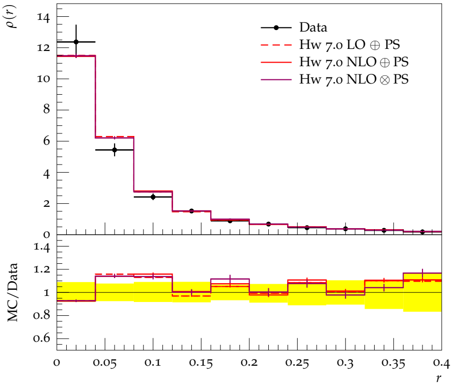
Differential jet shape for light-jets with 70 \text{ GeV} < p_T < 100 \text{ GeV}
