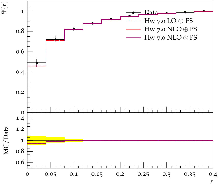
Integrated jet shape for light jets with 70 \text{ GeV} < p_T < 100 \text{ GeV}
