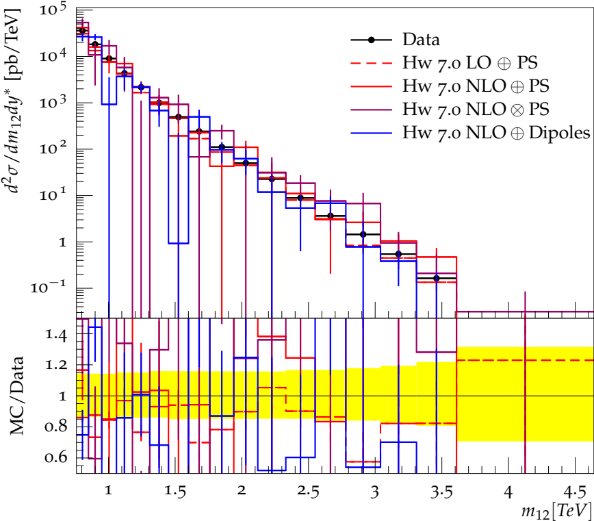
Dijet double-differential cross sections ( 1.5 < y^* < 2.0 ), R=0.4
