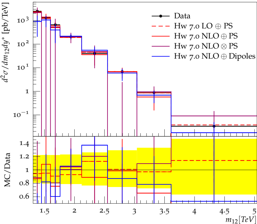
Dijet double-differential cross sections ( 2.0 < y^* < 2.5 ), R=0.4
