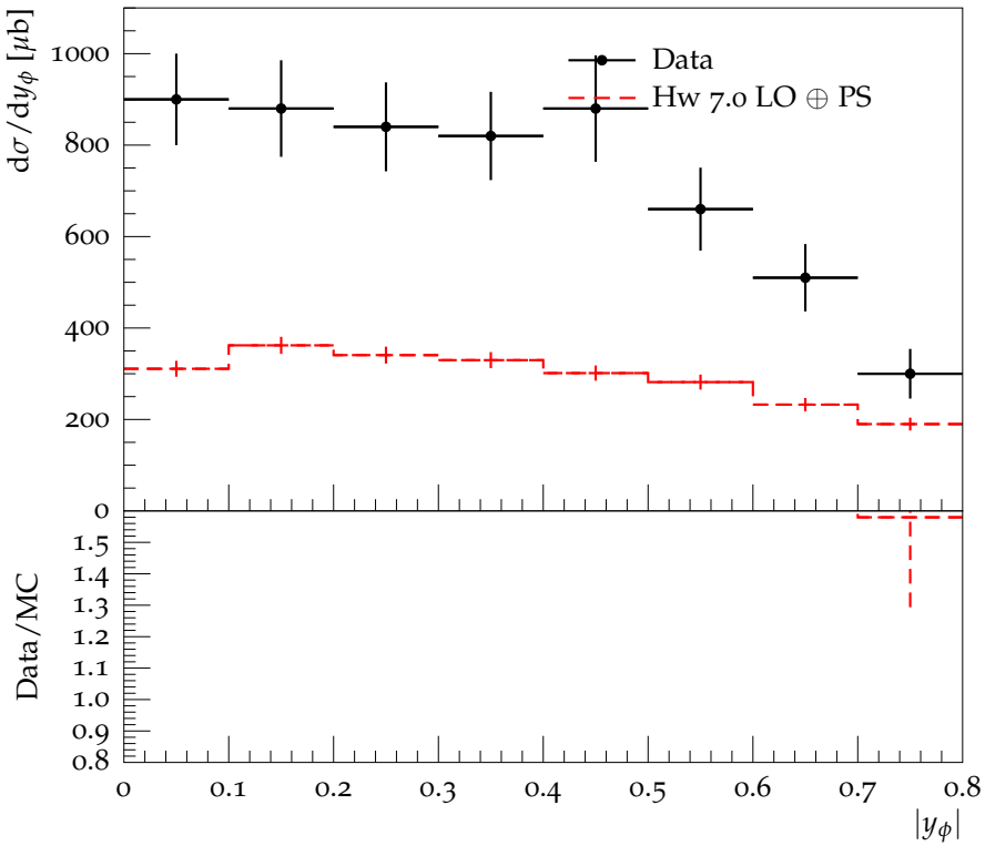
Fiducial \sigma(\phi \rightarrow K^+K^-) differential in |y_\phi|
