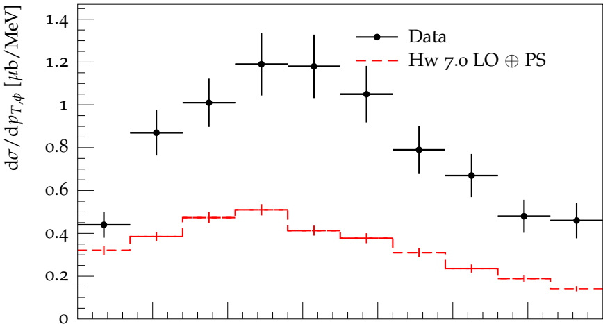
Fiducial \sigma(\phi \rightarrow K^+K^-) differential in p_{T,\phi}
