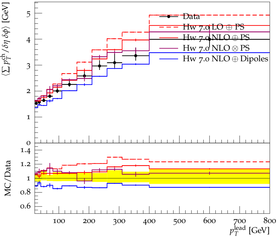
Trans-max \langle \sum p_T^{\text{ch}} / \delta\eta \delta\phi \rangle vs. p_T^{\text{lead}} in |\eta| < 2.5 in incl jet events
