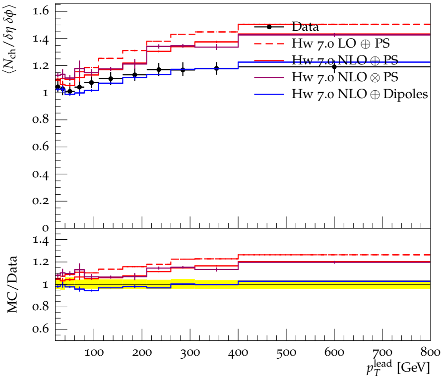
Transverse \langle N_{\text{ch}}/\delta\eta\delta\phi \rangle vs. p_T^{\text{lead}} in |\eta| < 2.5 in incl jet events
