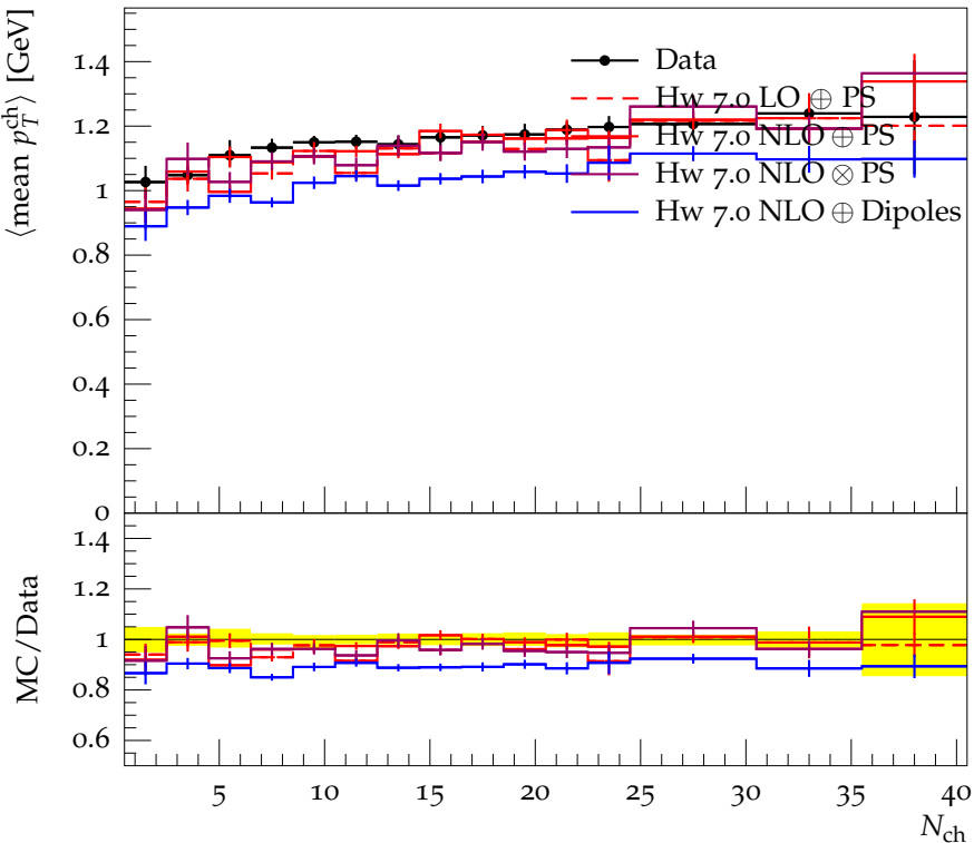
Transverse \langle \text{mean } p_T^{\text{ch}} \rangle vs. N_{\text{ch}} in |\eta| < 2.5 in incl jet events
