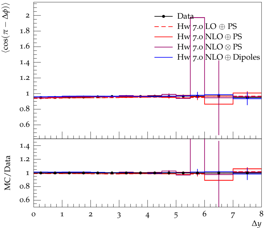
\langle \cos(\pi - \Delta\phi) \rangle for gap events as a function of \Delta\gamma
