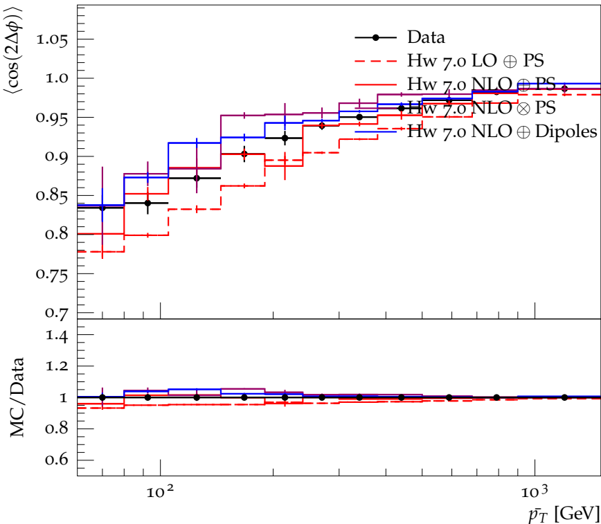
\langle \cos(2\Delta\phi) \rangle for gap events as a function of p_T
