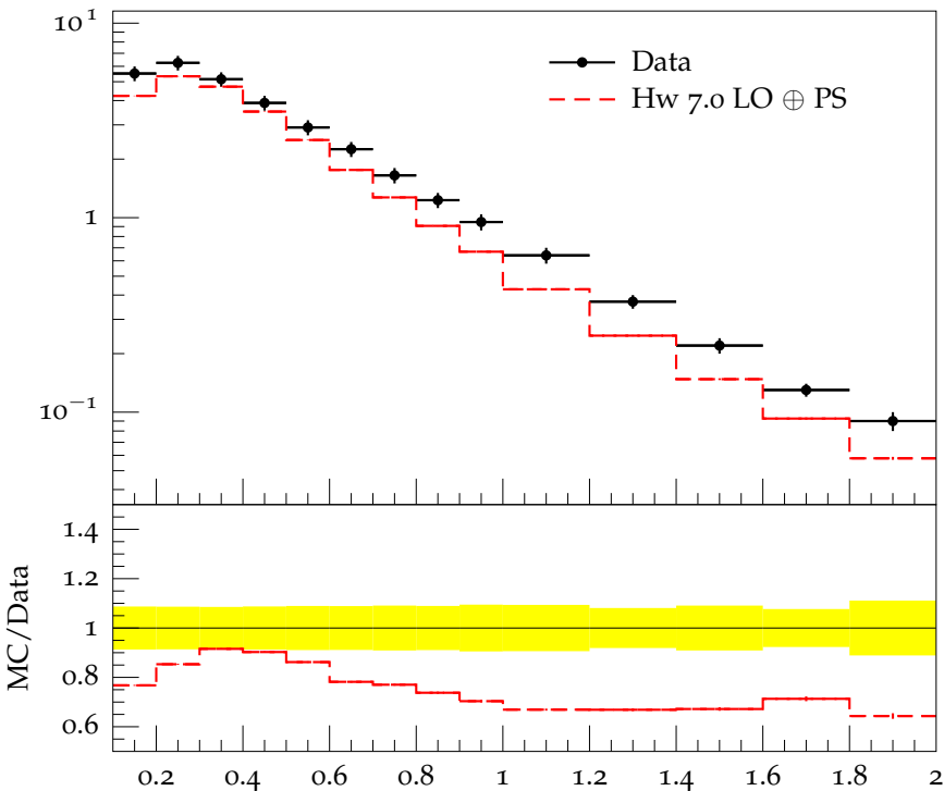
Charged hadron p_{\perp} for |\eta| = 0.1 at \sqrt{s} = 0.9 TeV
