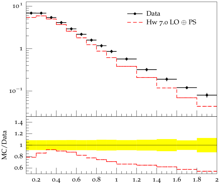
Charged hadron p_{\perp} for |\eta| = 1.9 at \sqrt{s} = 0.9 TeV
