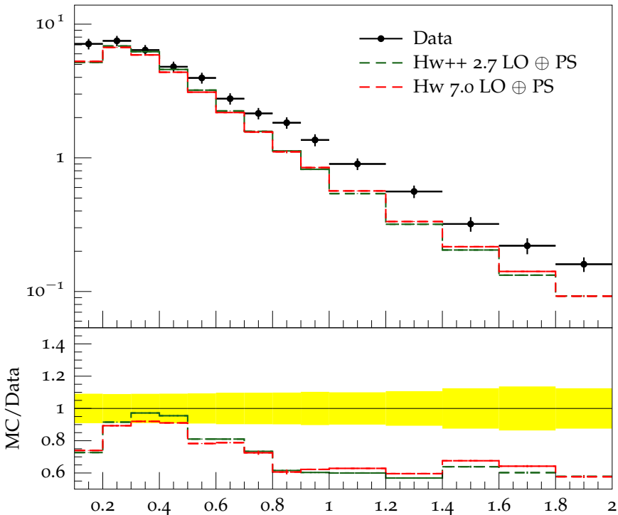
Charged hadron p_{\perp} for |\eta| = 0.1 at \sqrt{s} = 2.36 TeV
