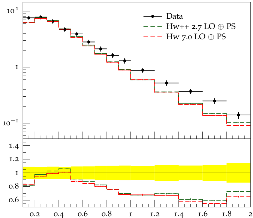
Charged hadron p_{\perp} for |\eta| = 1.1 at \sqrt{s} = 2.36 TeV
