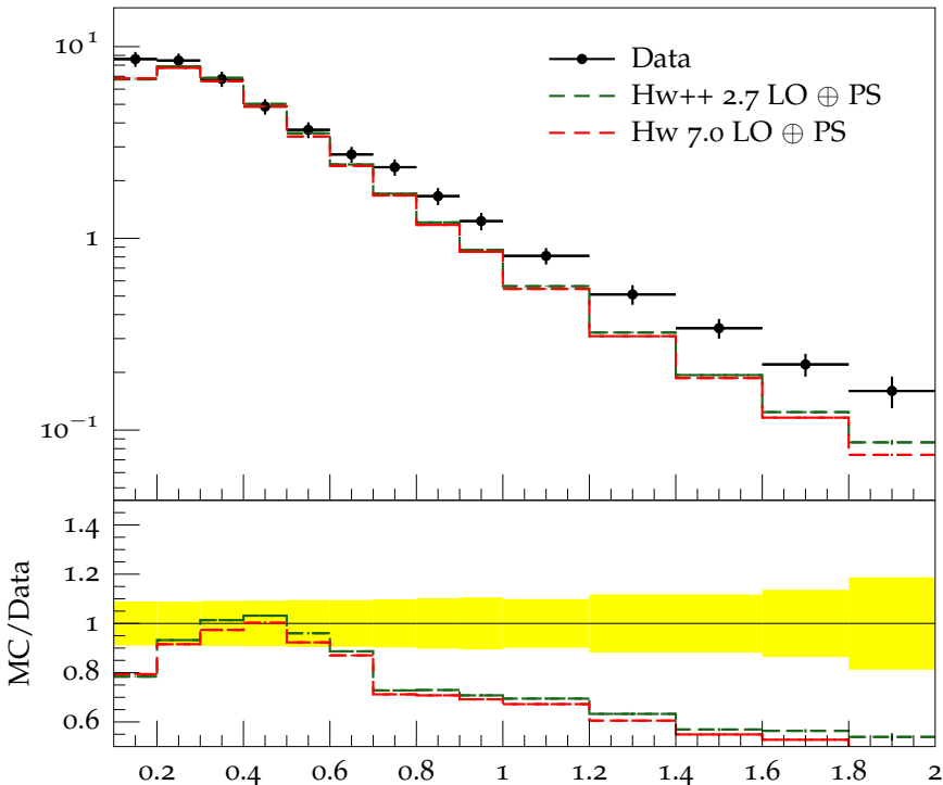
Charged hadron p_{\perp} for |\eta| = 1.7 at \sqrt{s} = 2.36 TeV
