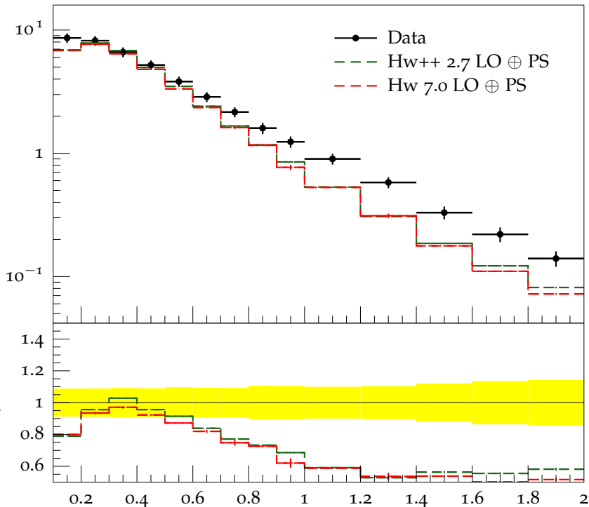
Charged hadron p_{\perp} for |\eta| = 1.9 at \sqrt{s} = 2.36 TeV
