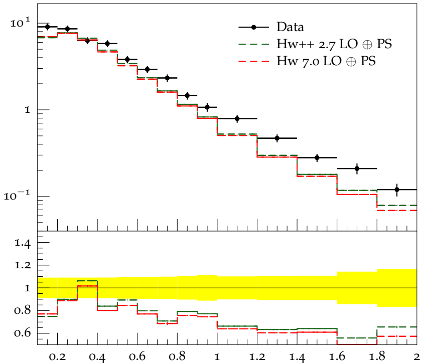
Charged hadron p_{\perp} for |\eta| = 2.1 at \sqrt{s} = 2.36 TeV
