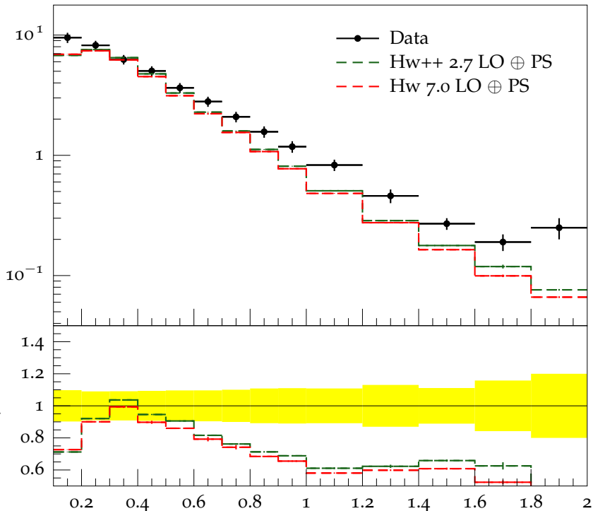
Charged hadron p_{\perp} for |\eta| = 2.3 at \sqrt{s} = 2.36 TeV
