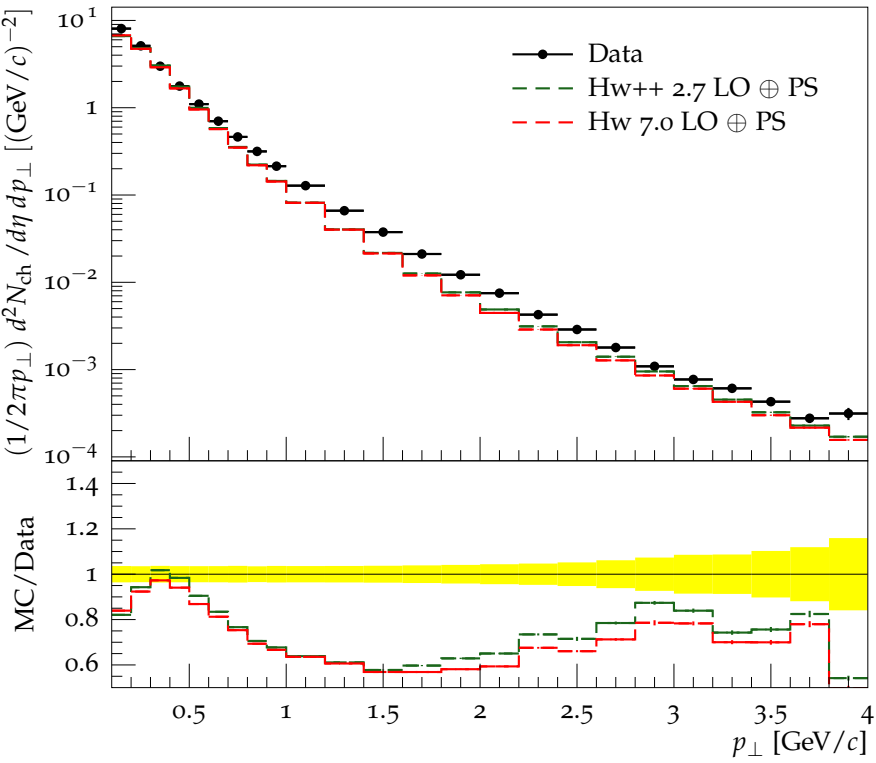
Charged hadron p_{\perp} for |\eta| < 2.4 at \sqrt{s} = 2.36 TeV
