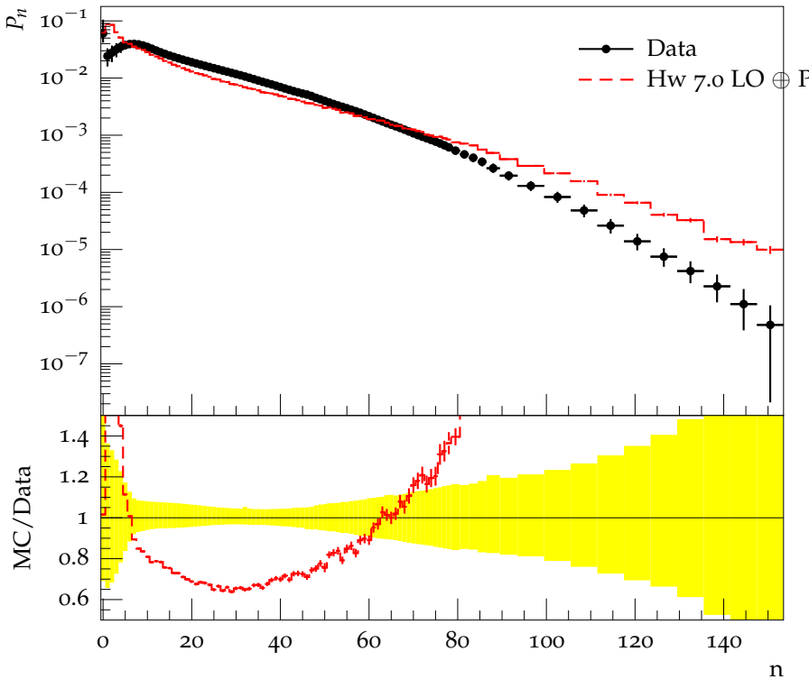
Charged hadron multiplicity, |\eta| < 1.5 , \sqrt{s} = 7 TeV
