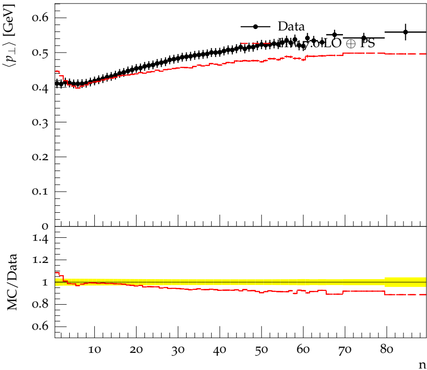
Mean p_{\perp} vs charged hadron multiplicity, |\eta| < 2.4 , \sqrt{s} = 0.9 TeV
