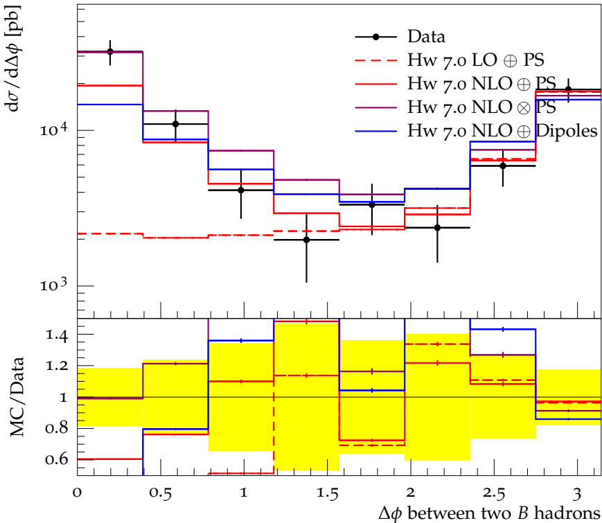
B\bar{B} production cross-section (leading jet p_{\perp} > 56 GeV)
