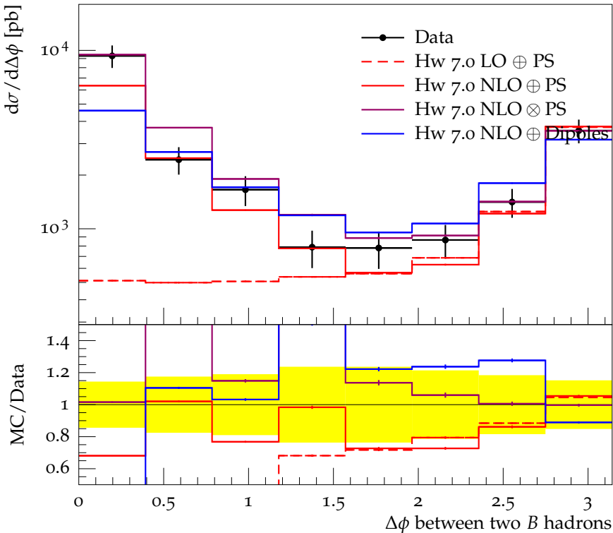
B\bar{B} production cross-section (leading jet p_{\perp} > 84 GeV)
