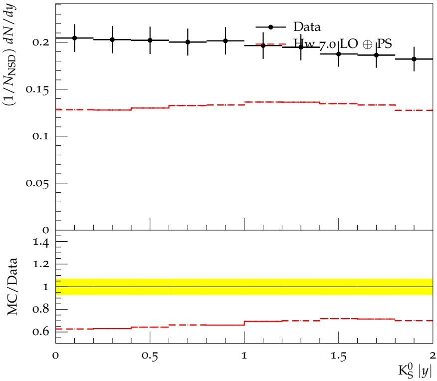
K_S^0 rapidity distribution at \sqrt{s} = 0.9 TeV
