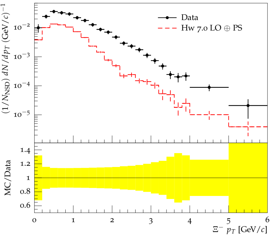
\Xi^- transverse momentum distribution at \sqrt{s} = 0.9 TeV
