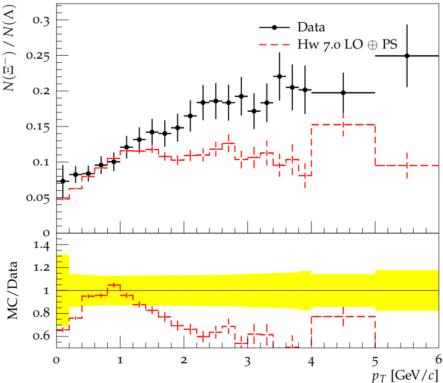
E^- / \Lambda versus transverse momentum at \sqrt{s} = 7 TeV
