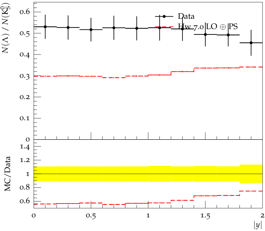
\Lambda/K_S^0 versus rapidity at \sqrt{s} = 0.9 TeV
