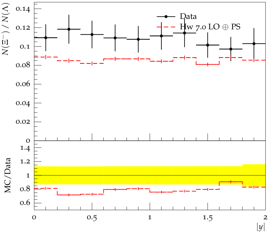
E^- / \Lambda versus rapidity at \sqrt{s} = 7 TeV
