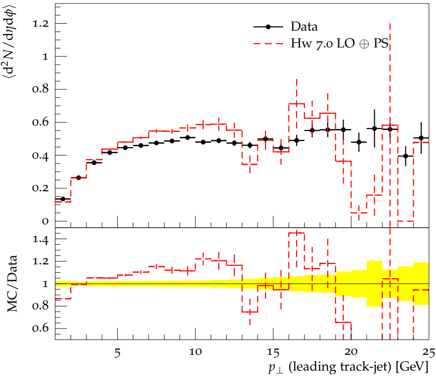
Transverse N_{\text{ch}} density vs. p_{\perp}^{\text{jet } 1} , \sqrt{s} = 900 \text{ GeV}
