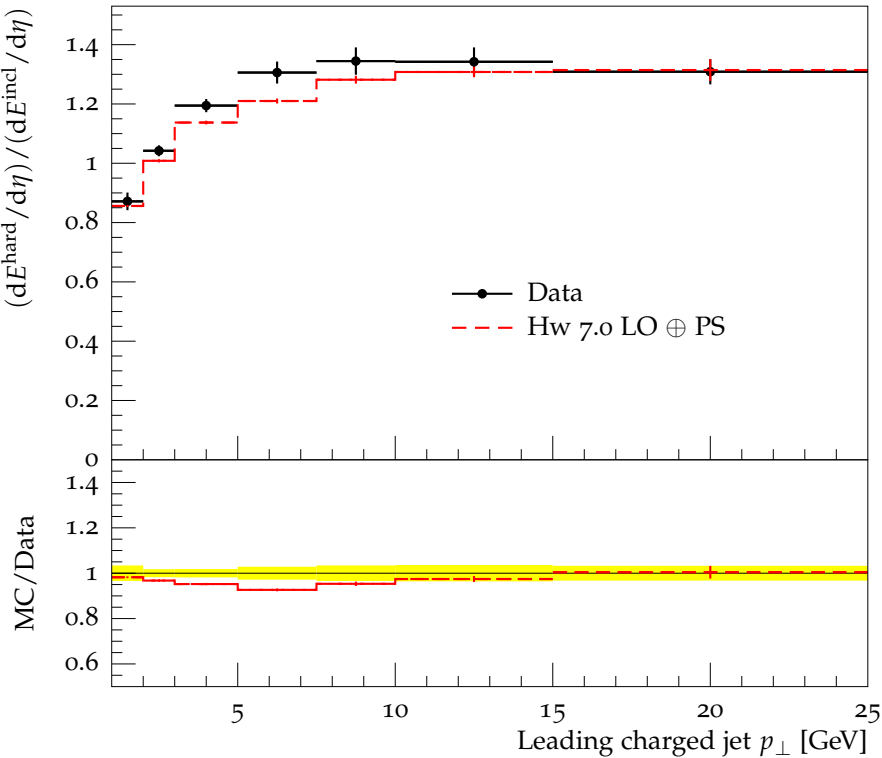
Ratio of energy deposited in -6.6 < \eta < -5.2 for \sqrt{s} = 7 TeV
