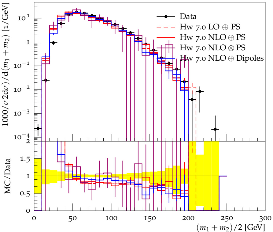
Filtered AK7 dijets, (p_T^1 + p_T^2)/2 = 500\text{--}600 GeV
