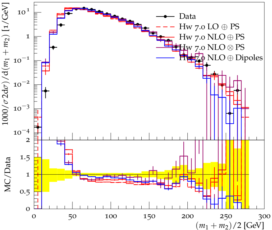
Filtered AK7 dijets, (p_T^1 + p_T^2)/2 = 600\text{--}800 GeV
