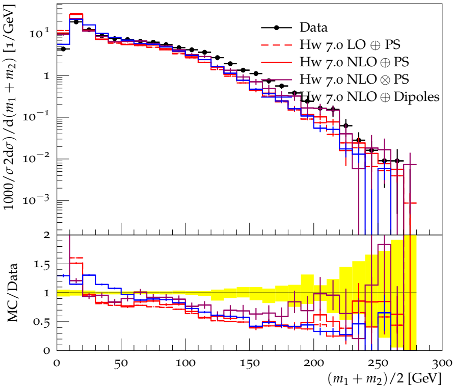
Pruned AK7 dijets, (p_T^1 + p_T^2)/2 = 600\text{--}800\text{ GeV}
