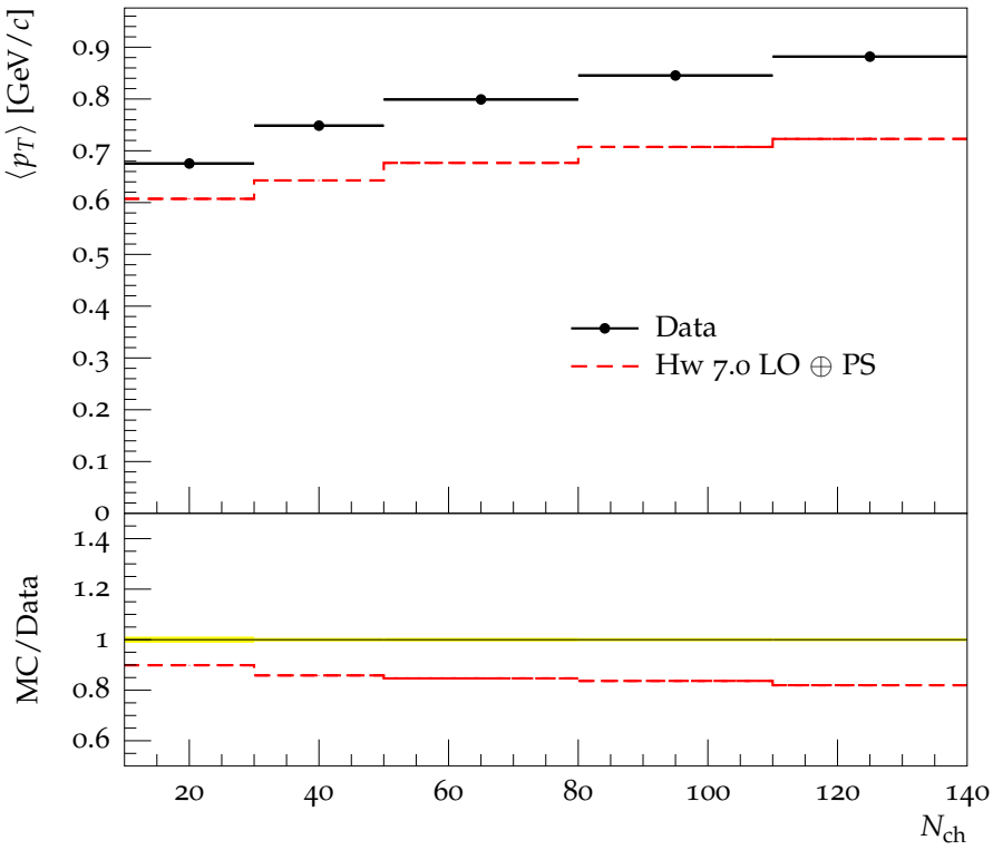
Mean p_{\perp} , all charged particles
