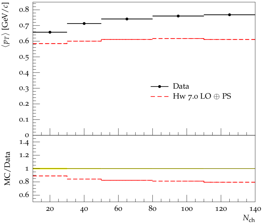
Mean p_{\perp} , UE charged particles
