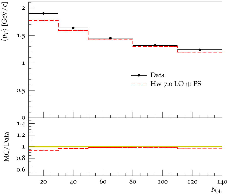
Mean p_{\perp} , in-jet charged particles
