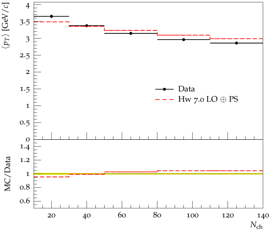
Mean p_{\perp} , leading in-jet charged particle
