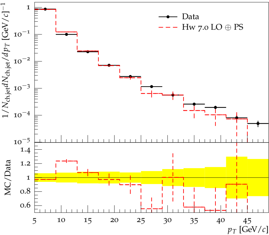
Jet p_T spectrum, |\eta^{ch.jet}| < 1.9, 30 < N_{ch} \leq 50
