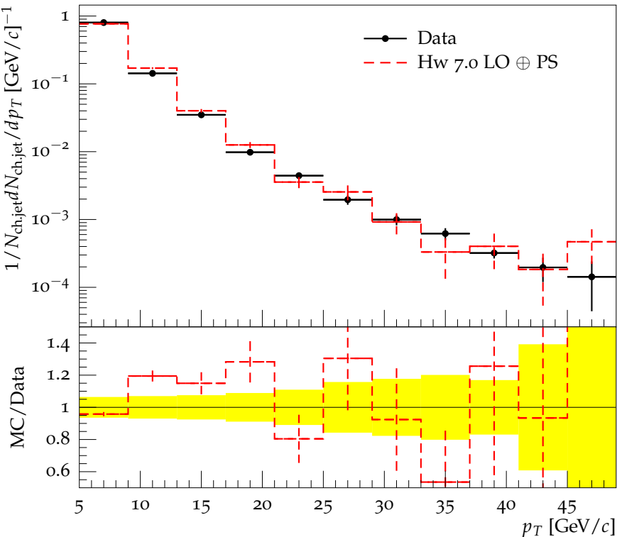
Jet p_T spectrum, |\eta^{ch.j\text{et}}| < 1.9 , 110 < N_{\text{ch}} \leq 140
