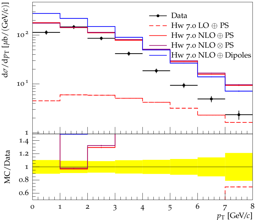
Prompt D^0 + \text{c.c.} d\sigma/dp_T for rapidity interval 2.0 < y < 2.5
